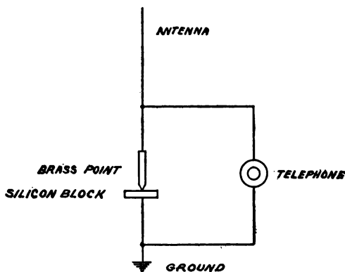
FIG. 17.—CONNECTIONS OF SILICON DETECTOR.
